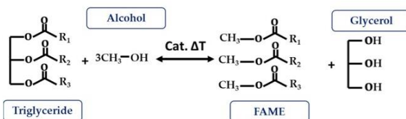
Figure 6. Transesterification reaction.
