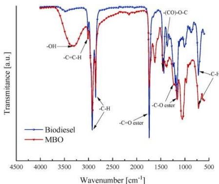
Fig. 6. FTIR spectra of bio-oil and biodiesel.
