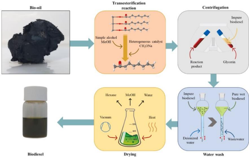
Fig. 3. Biodiesel purification process after transesterification.
